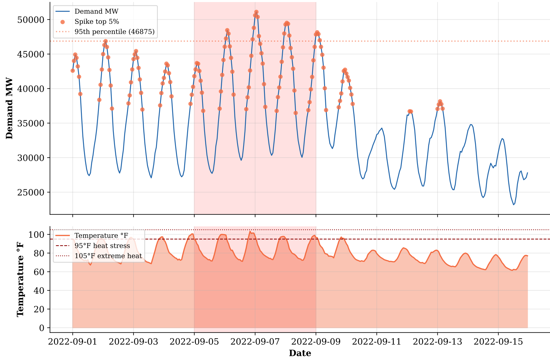
Figure 4: California Grid Stress and Temperature — September 2022 Heat Wave Extreme temperatures coincide with spike events outside normal conditions
