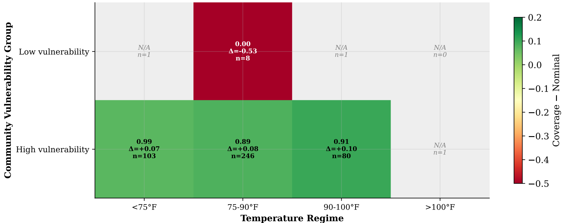
Figure 6: Coverage Degradation by Vulnerability × Temperature Regime Nominal coverage = 90%. Red = under-coverage. Asterisk = fallback for sparse subgroup cell.
