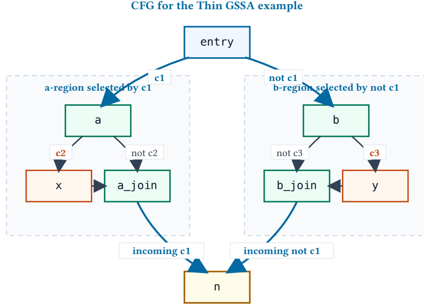
Figure 3: CFG for the Thin GSSA example. The incoming regions for the phi at n are selected by c1 and \text{not } c1 . The local branches c2 and c3 only choose paths inside those regions before they reconverge at a\_join and b\_join .
