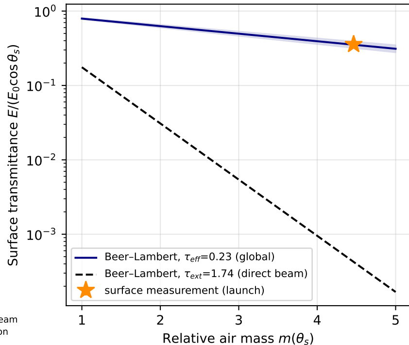
(b) Beer-Lambert attenuation curves
