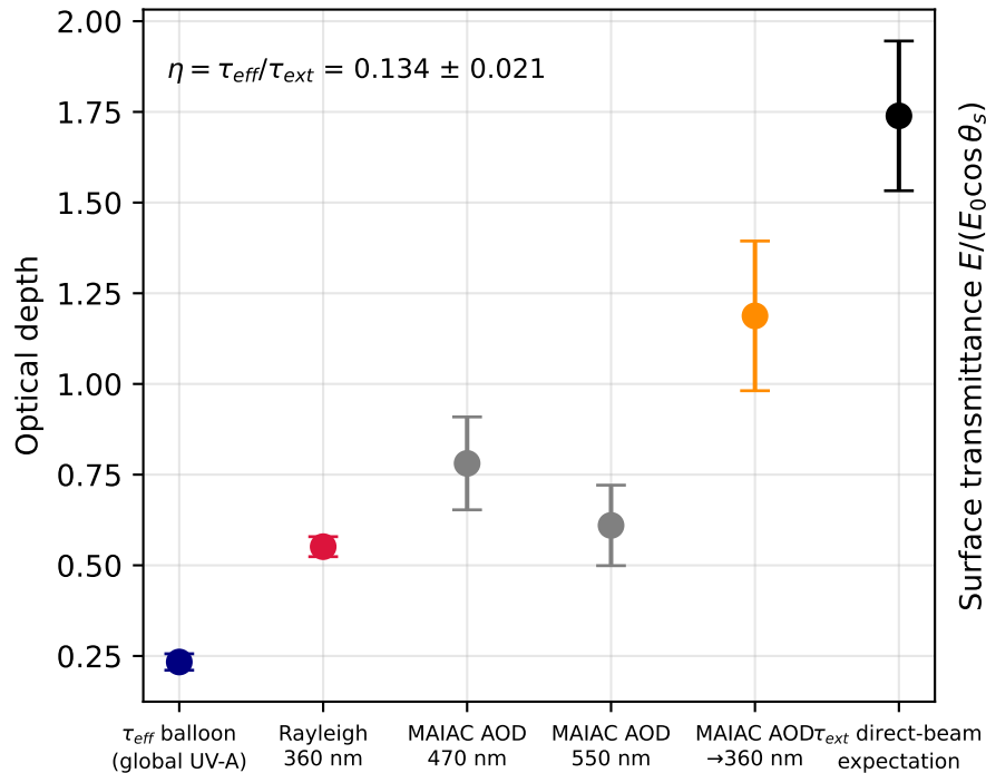
(a) Column optical depths, 5 Oct 2025
