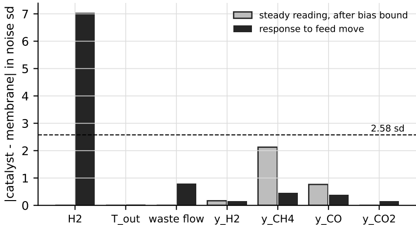
Mode 1, 5% H2 drop: catalyst ( a_c=0.673 ) vs membrane ( a_m=0.949 )
