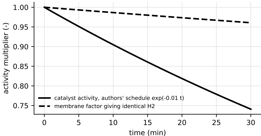
Same H 2 signal, very different underlying loss (Mode 1, constant feed)
