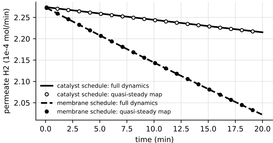
Validation V1: quasi-steady map vs full dynamics (Mode 1)
