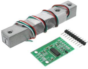
Fig. 12. HX711 & Straight Bar Load Cell
