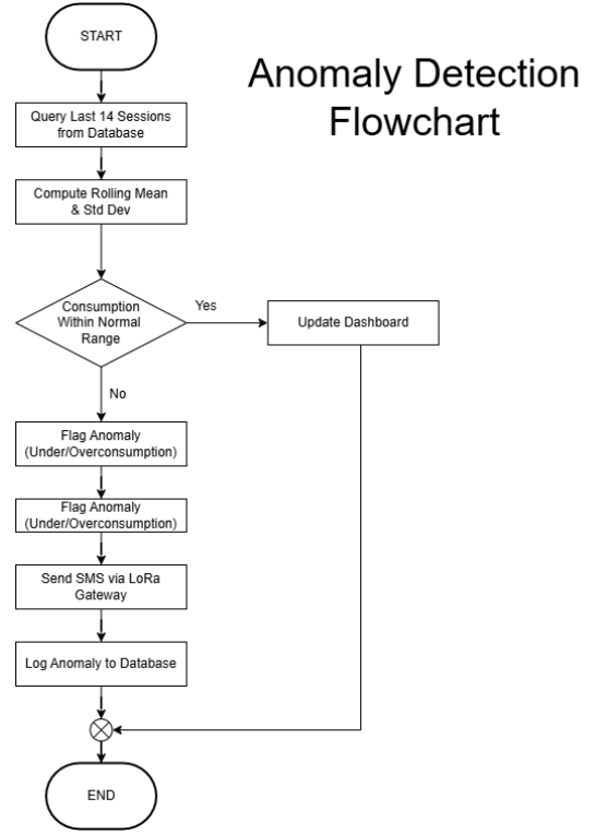
Fig. 21. Anomaly Detection Flowchart
