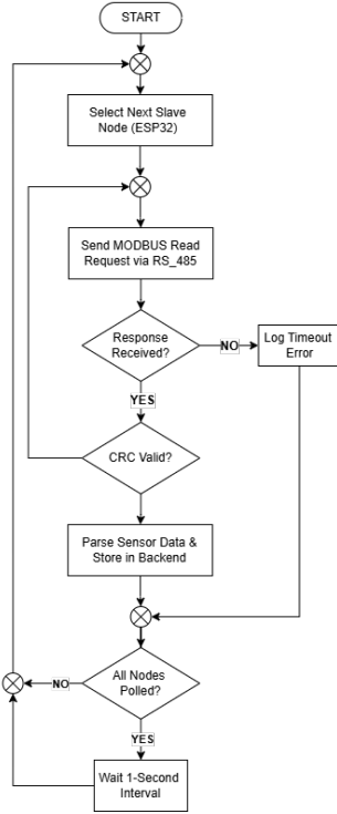
Fig. 16. RS-485 / MODBUS RTU Communication Flowchart
