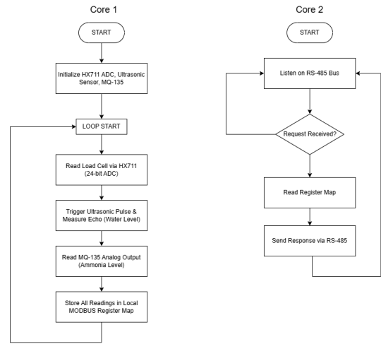
Fig. 5. ESP32 Edge Node Firmware Flowchart (Dual-Core)
