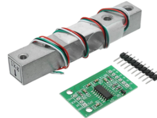
Fig. 12. HX711 & Straight Bar Load Cell
