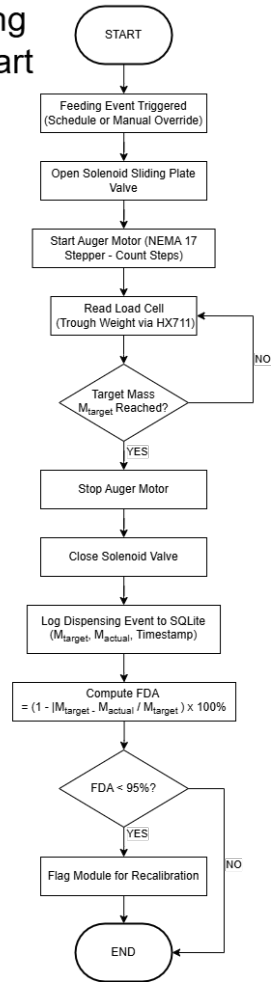
Fig. 11. Feed Dispensing Module Flowchart
