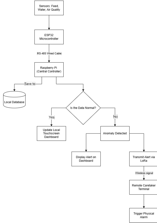
Fig. 2. System Flowchart
