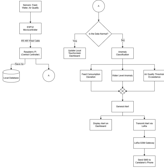
Fig. 2. System Flowchart
