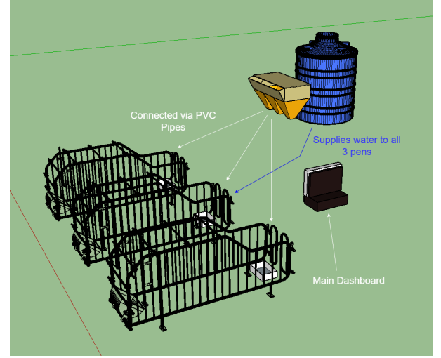
Fig. 3. 3D Visualization of the System Deployment in a Piggery Environment
