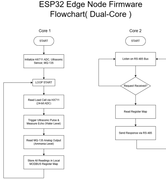
Fig. 5. ESP32 Edge Node Firmware Flowchart (Dual-Core)
