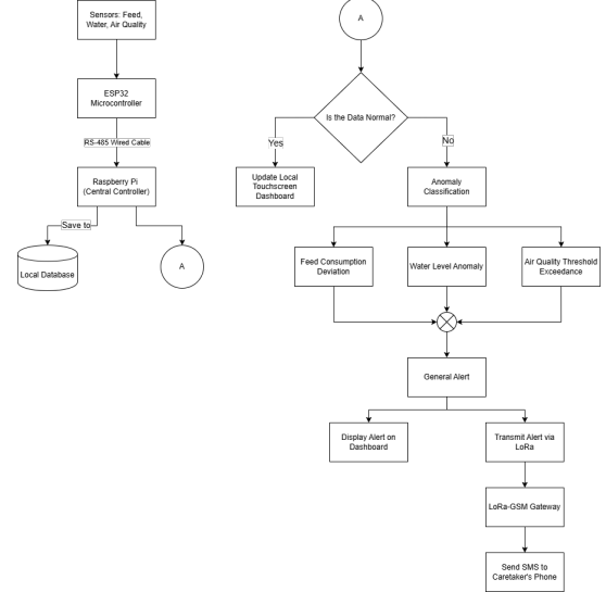
Fig. 2. System Flowchart
