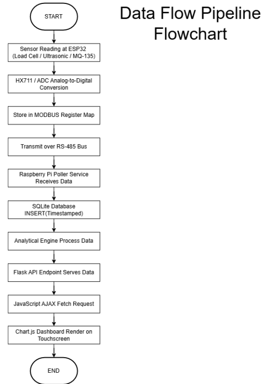
Fig. 4. Data Flow Pipeline Flowchart
