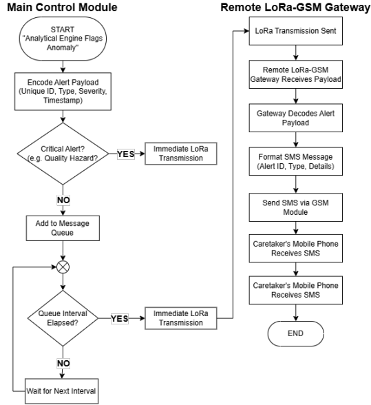
Fig. 17. LoRa-SMS Alert Pipeline Flowchart
