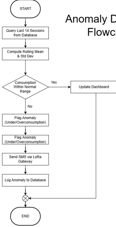
Fig. 20. Anomaly Detection Flowchart
