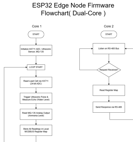
Fig. 4. ESP32 Edge Node Firmware Flowchart (Dual-Core)
