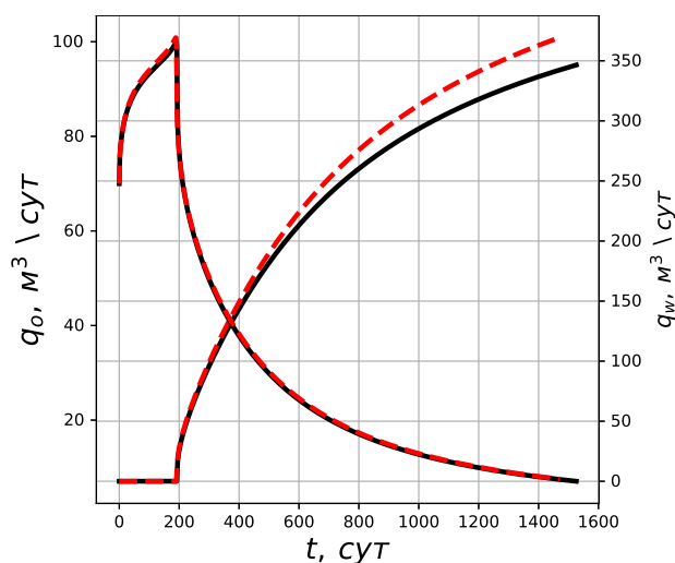
Rates of water and oil from the producing well
