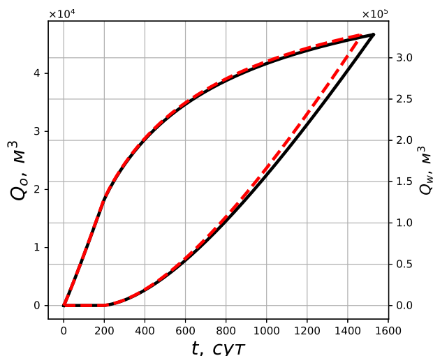
Accumulated rates of water and oil from the producing well
