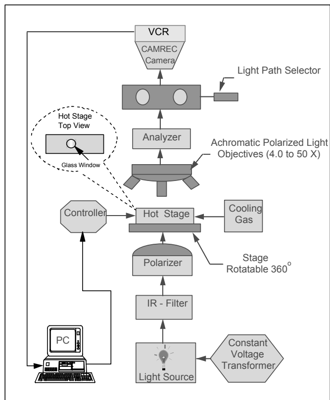
Fig. 1-Schematic of the Cross Polarized Microscope (CPM)
