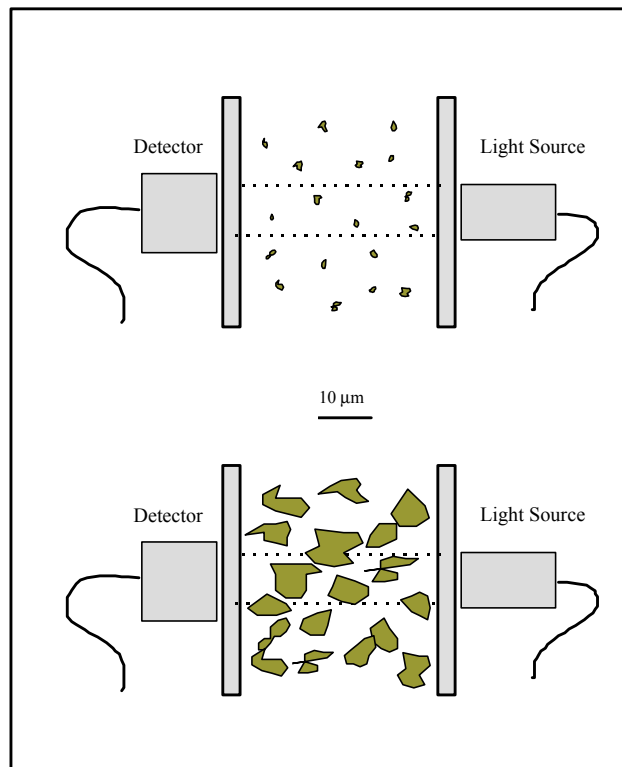
Fig. 9-Schematic illustration of the effect of wax crystal size on the transmitted light
