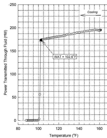
Fig. 6-Power of transmitted light through HI 557/well A-1 STO at 1 atm (cooling rate ~ 1°F/min).
