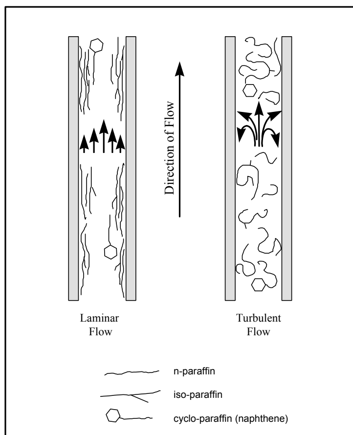
Fig. 11-Schematic illustrations of flow regimes in production wells and their effects on paraffin deposition.
