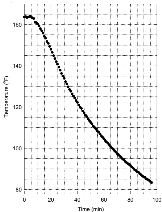
Fig. 3-Typical cooling curve for the solids detection system
