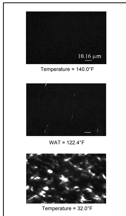
Fig. 5-CPM photomicrographs of HI 557/well A-1 STO at different temperatures (cooling rate = 1.8°F/min)
