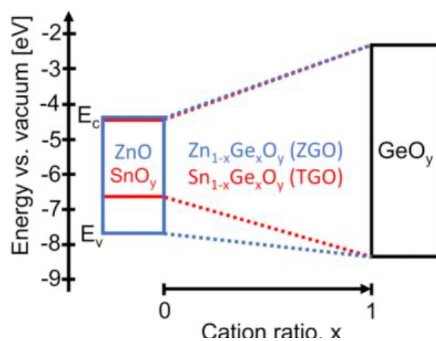
band diagram:
