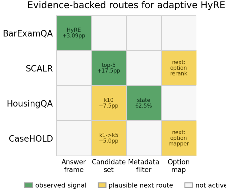
Figure 7: Route map implied by current evidence. Green cells are supported by observed route evidence; amber cells are plausible next interventions. The diagnostic protocol generalizes, while the current effects remain scoped to the model, task, and sample sizes reported above.
