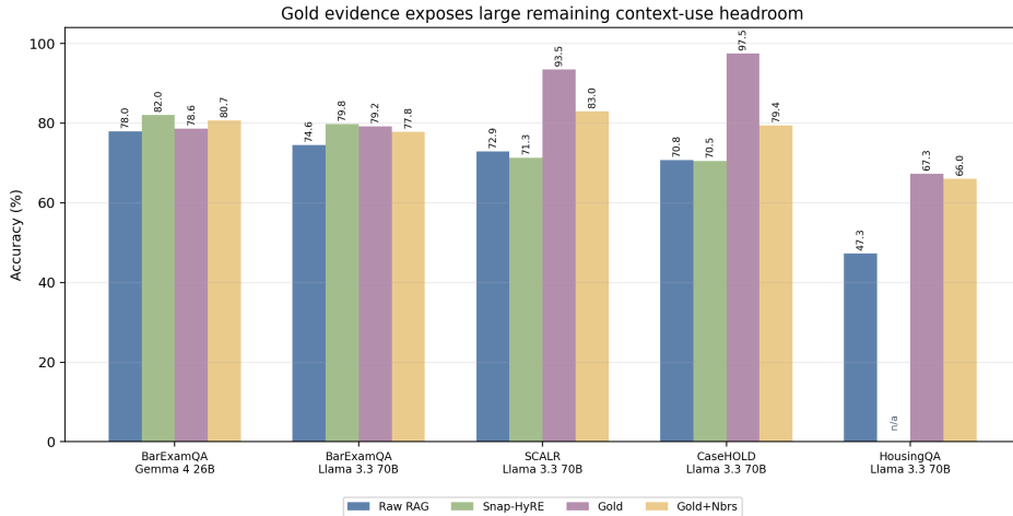
Figure 4: Oracle evidence controls expose remaining context-use headroom. Gold-plus-neighbor rows should not be read as an oracle ceiling; they also test distractor sensitivity.
