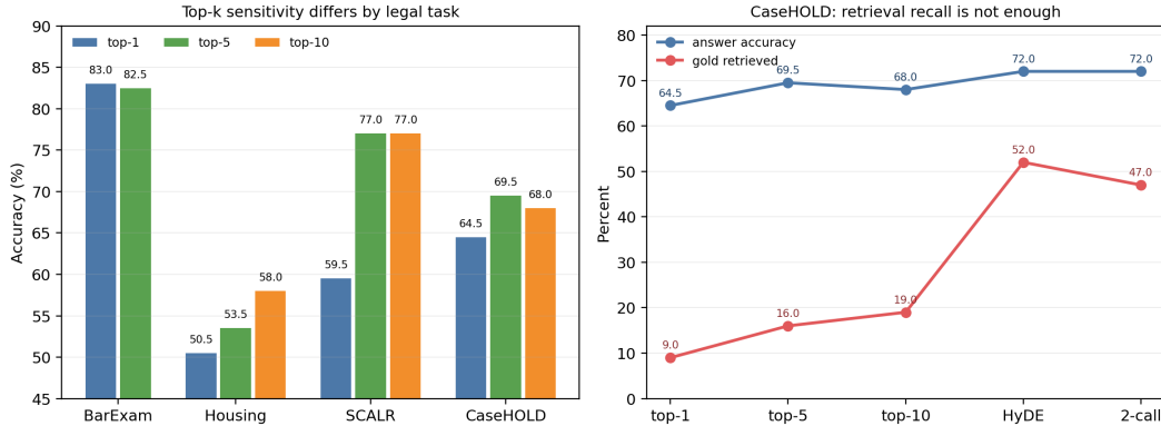
Figure 3: Legal benchmarks expose different bottlenecks. BarExamQA is depth-flat, SCALR benefits sharply from top-5 candidates, HousingQA has a directional top-10 signal, and CaseHOLD shows that gold-option retrieval can improve faster than answer accuracy.
