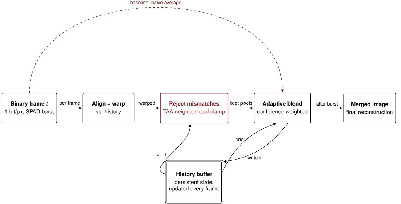
Figure 1: Per frame, the TAA-augmented pipeline (solid) warps the incoming binary frame to align with the running history buffer, rejects pixels where that alignment is unreliable, and adaptively blends the rest back into the history, which feeds the next frame and, after the full burst, the final reconstruction. The naive-averaging baseline (dashed) instead accumulates every frame directly, with no alignment or rejection.
