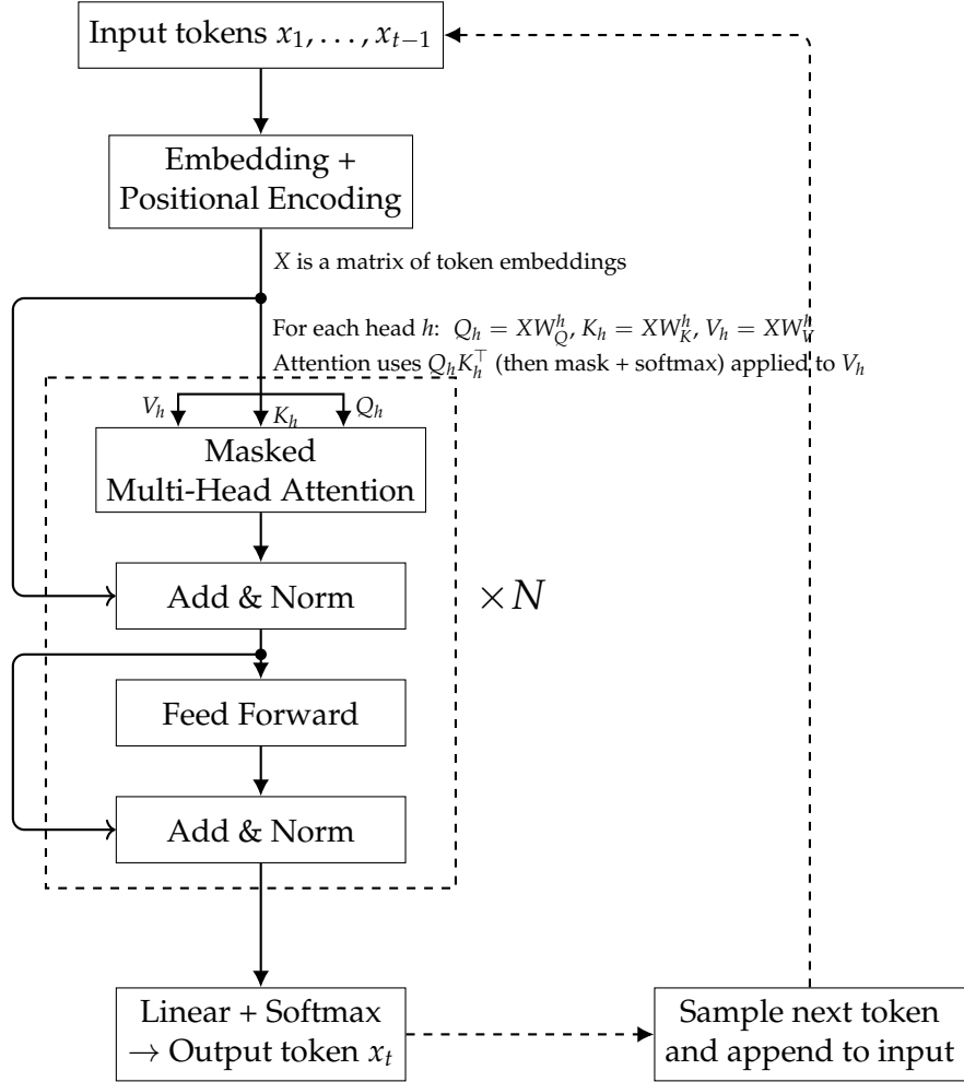
Figure A.1: Simplified architecture of a decoder-only transformer model for language modeling. Adapted from [vaswaniAttentionAllYou2017].
