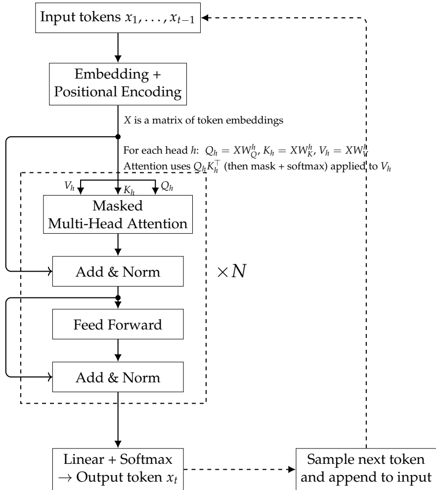
Figure 2.1: Simplified architecture of a decoder-only transformer model for language modeling. Adapted from [104].
