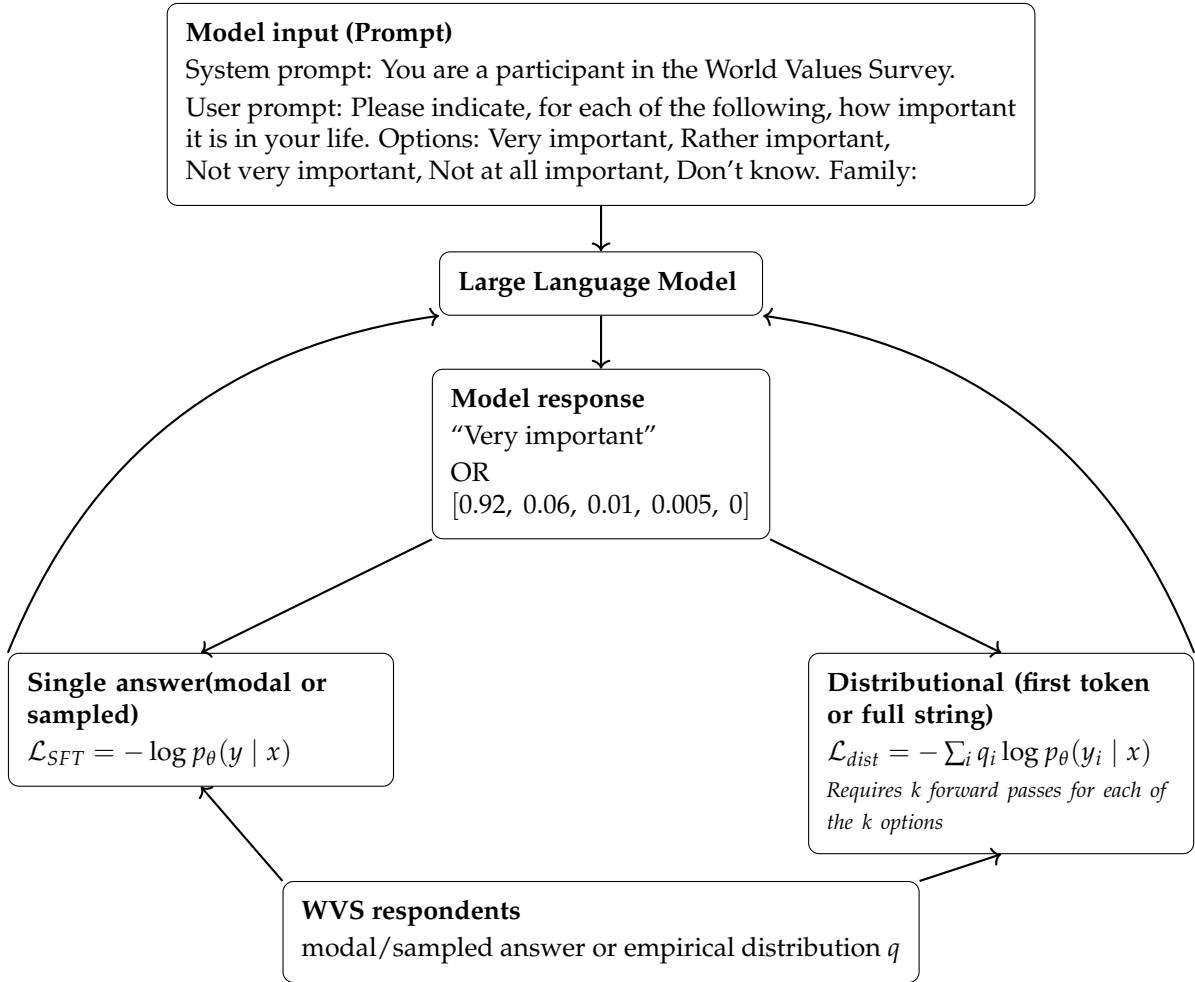
Figure 3.6: Simplified illustration of the fine-tuning setup. The model is prompted with a system persona and a survey question with its response options, and its response is used in two different loss functions: a simple SFT loss against the single modal (or sampled) answer, and a distributional loss against the full distribution of responses from the WVS respondents.
