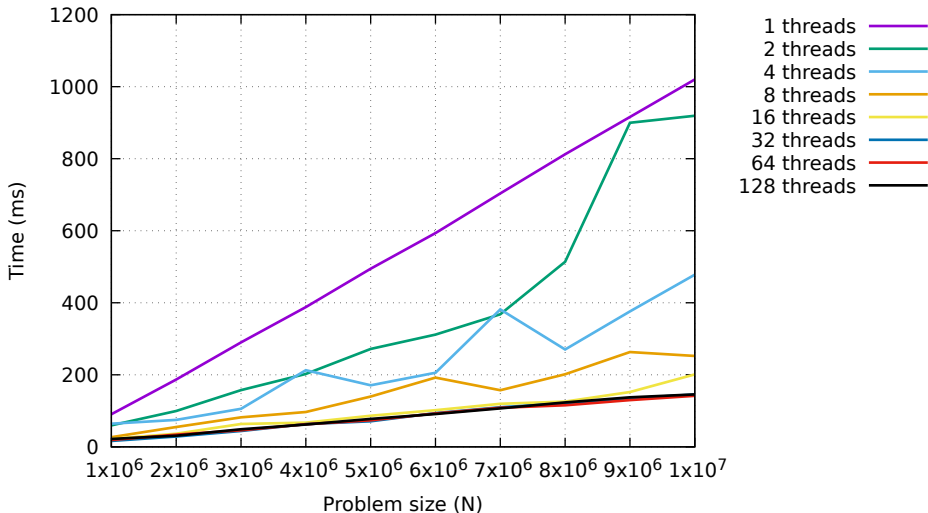
Quicksort: Average Time vs Problem Size
