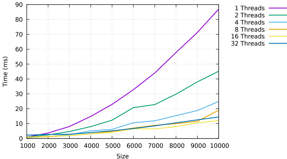
Average Execution Time vs Problem Size - CPU has 16 threads
