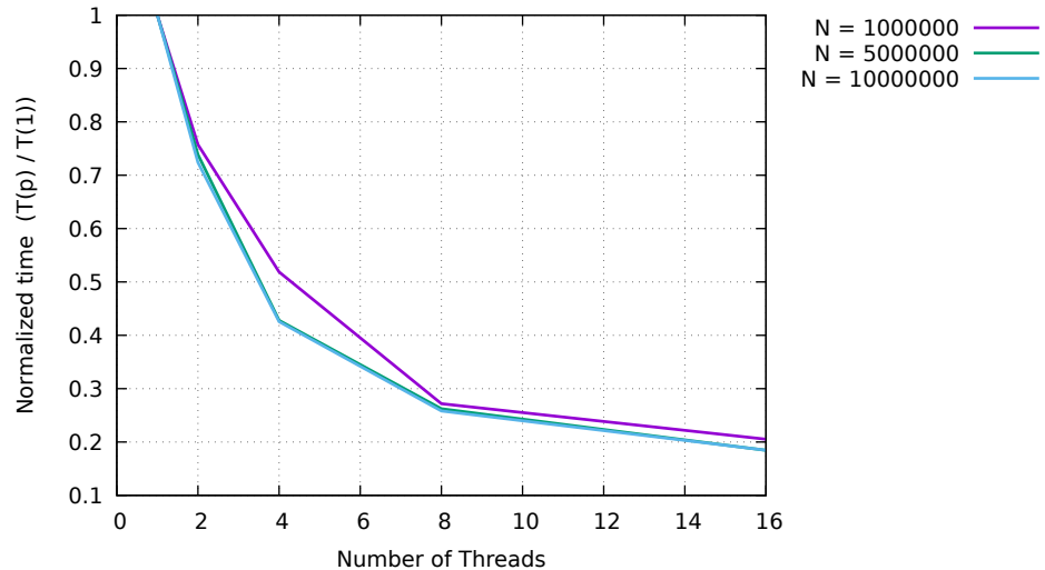
Normalized Execution Time vs Threads
