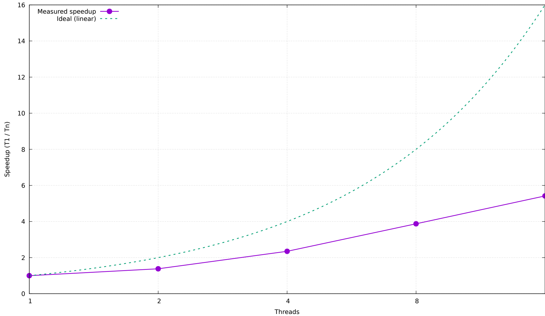
Quicksort Speedup
