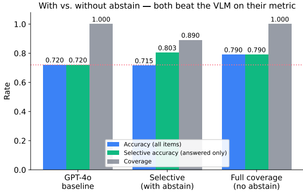
Figure 3: SEA vs. the GPT-4o baseline. The full-coverage model improves raw accuracy (+7.0 pts); the selective model exceeds the baseline in selective accuracy while answering 89.0% of items with verified evidence.
