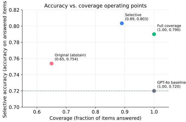
Figure 9: Operating points in the coverage/accuracy plane. Both SEA configurations sit above the GPT-4o baseline; the selective point answers 89.0% of items at higher selective accuracy.
