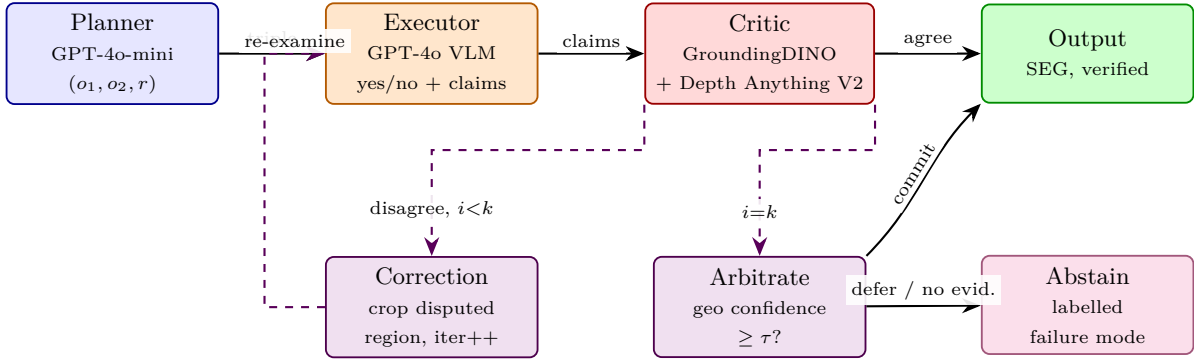
Figure 1: SEA pipeline. Three specialised agents communicate through a typed AgentState. The correction loop zooms into the disputed region for up to k re-examinations; when the budget is exhausted, the arbitration node commits geometry, defers to the VLM, or abstains based on geometric confidence.
