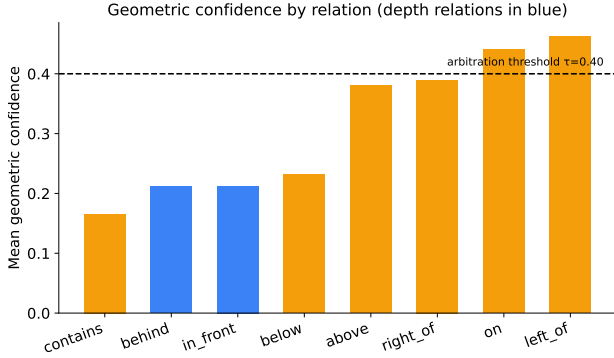
Figure 2: Mean geometric confidence by relation. Depth relations (blue) and the non-separable contains relation fall below the arbitration threshold \tau = 0.40 and defer to the VLM; well-separated position relations clear it and can commit geometry.
