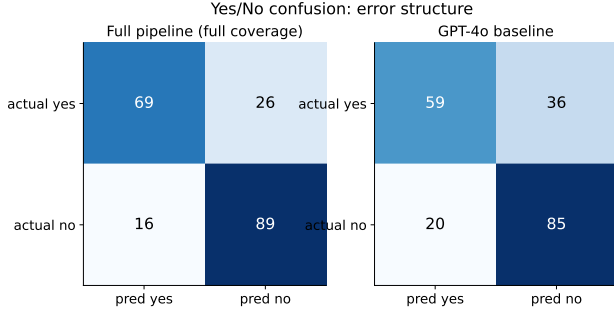
Figure 6: Yes/No confusion. SEA (left) recovers 10 more true “yes” answers than the baseline (right) at lower false-positive cost.
