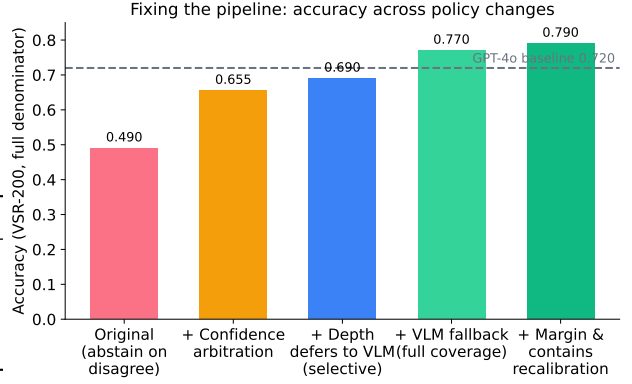
Figure 4: Accuracy across reconciliation-policy design steps. Each change moves SEA upward; the final full-coverage policy crosses the GPT-4o baseline. The gain is driven by how disagreements are reconciled, not by changing the underlying detector or depth model.
