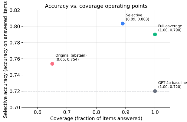
Figure 9: Operating points in the coverage/accuracy plane. Both SEA configurations sit above the GPT-4o baseline; the selective point answers 89.0% of items at higher selective accuracy.
