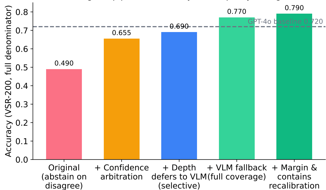
Fixing the pipeline: accuracy across policy changes
