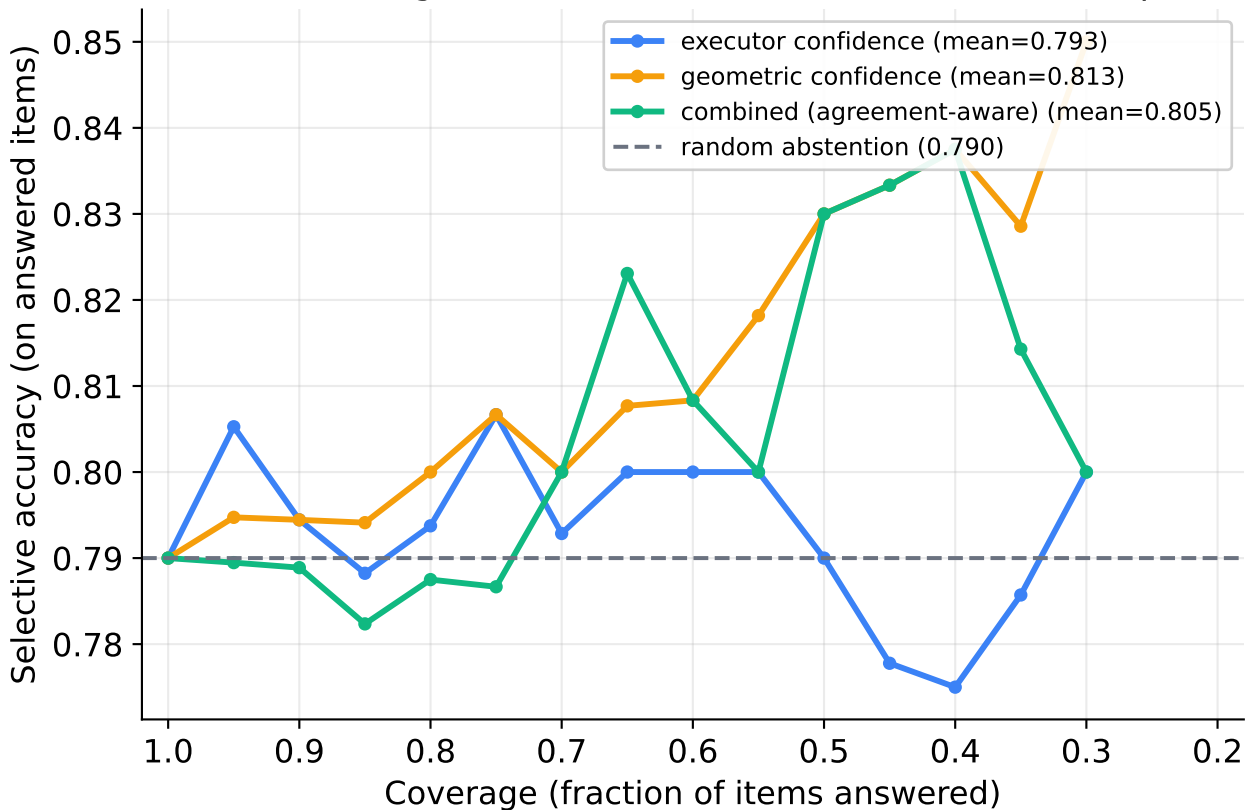
Risk-coverage: does confidence-based abstention help?
