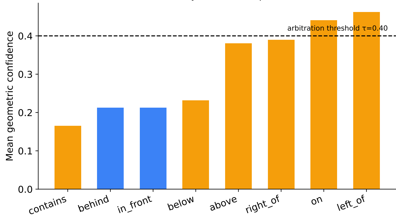
Geometric confidence by relation (depth relations in blue)
