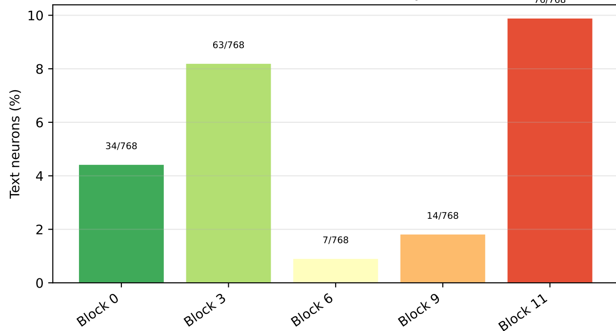
(a) CLIP ViT-B/32: text-neuron fraction by transformer block
