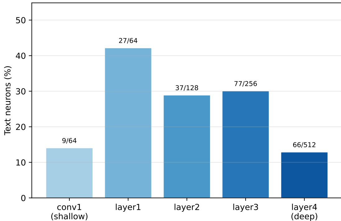
(a) MILAN text-neuron fraction by layer depth
