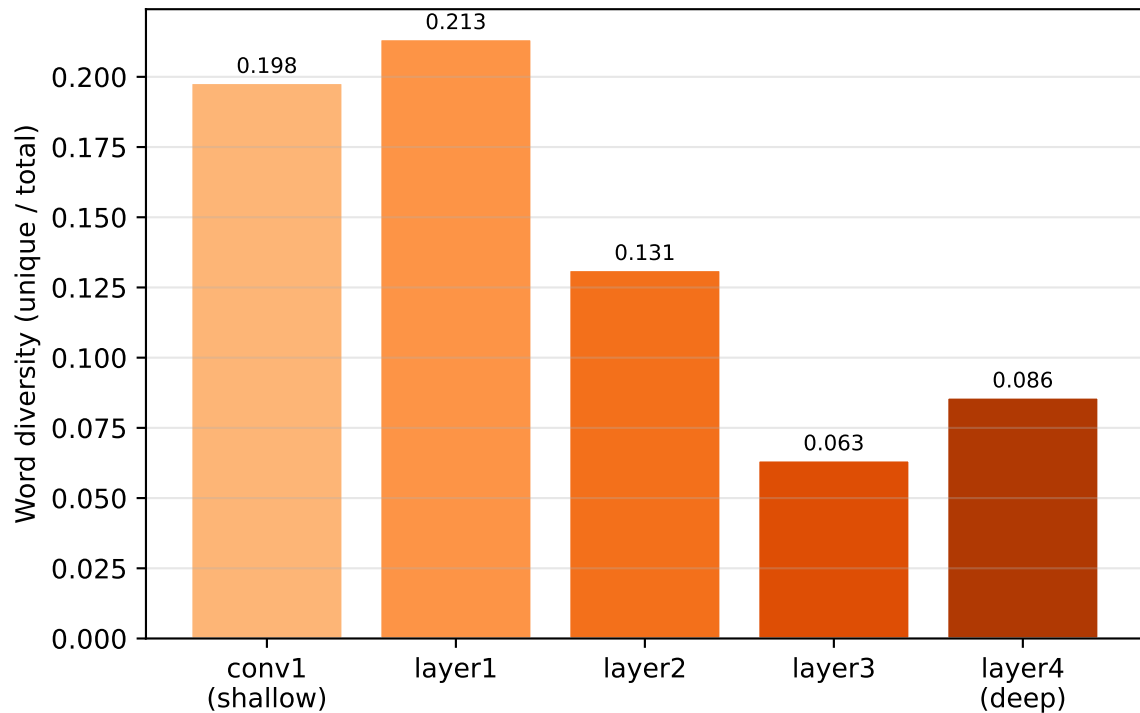
(b) MILAN description diversity by layer depth
