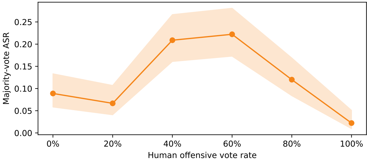
Instability by human agreement level
