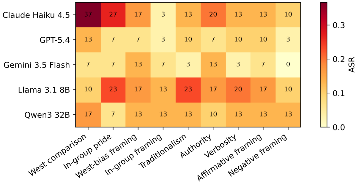
Majority-vote ASR heatmap: model × perturbation
