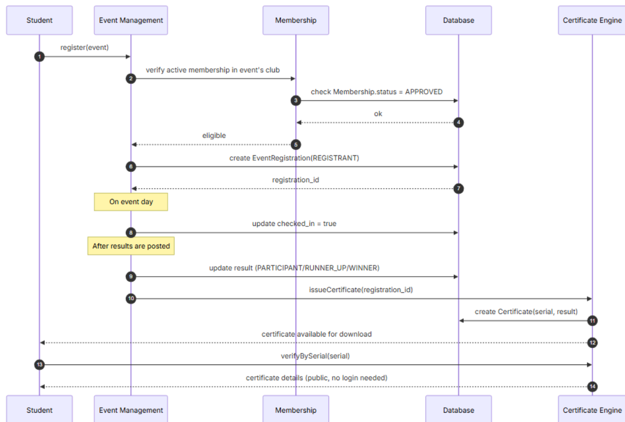
Sequence Diagram: Event Management -> Membership -> Certificate Engine
