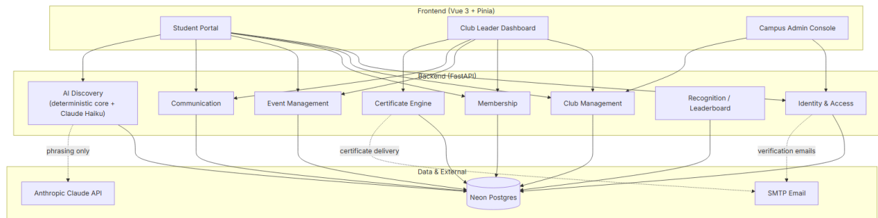
Campus Connect - System Component / Architecture Diagram
