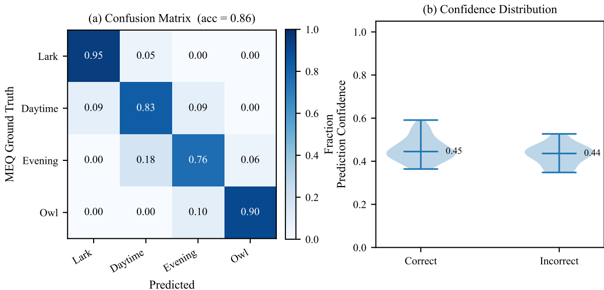
Fig. 2 — Chronotype Classification Accuracy [Synthetic (n=80)]
