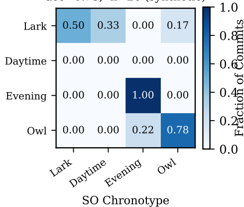
(a) Cross-Modal Agreement acc=0.75, n=20 (synthetic)
