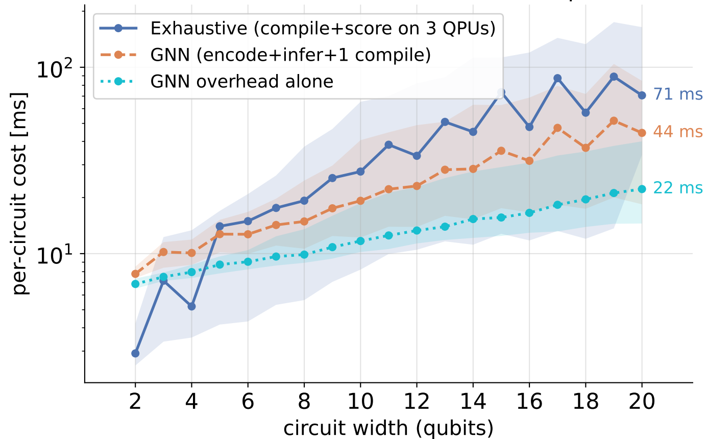
Device-selection cost: exhaustive vs GNN-predicted
