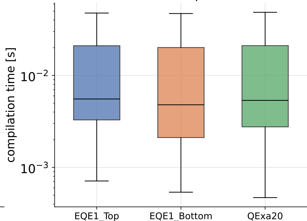
Per-backend compilation time
