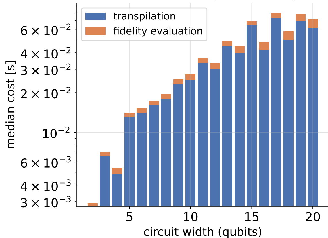
Cost breakdown (all backends)
