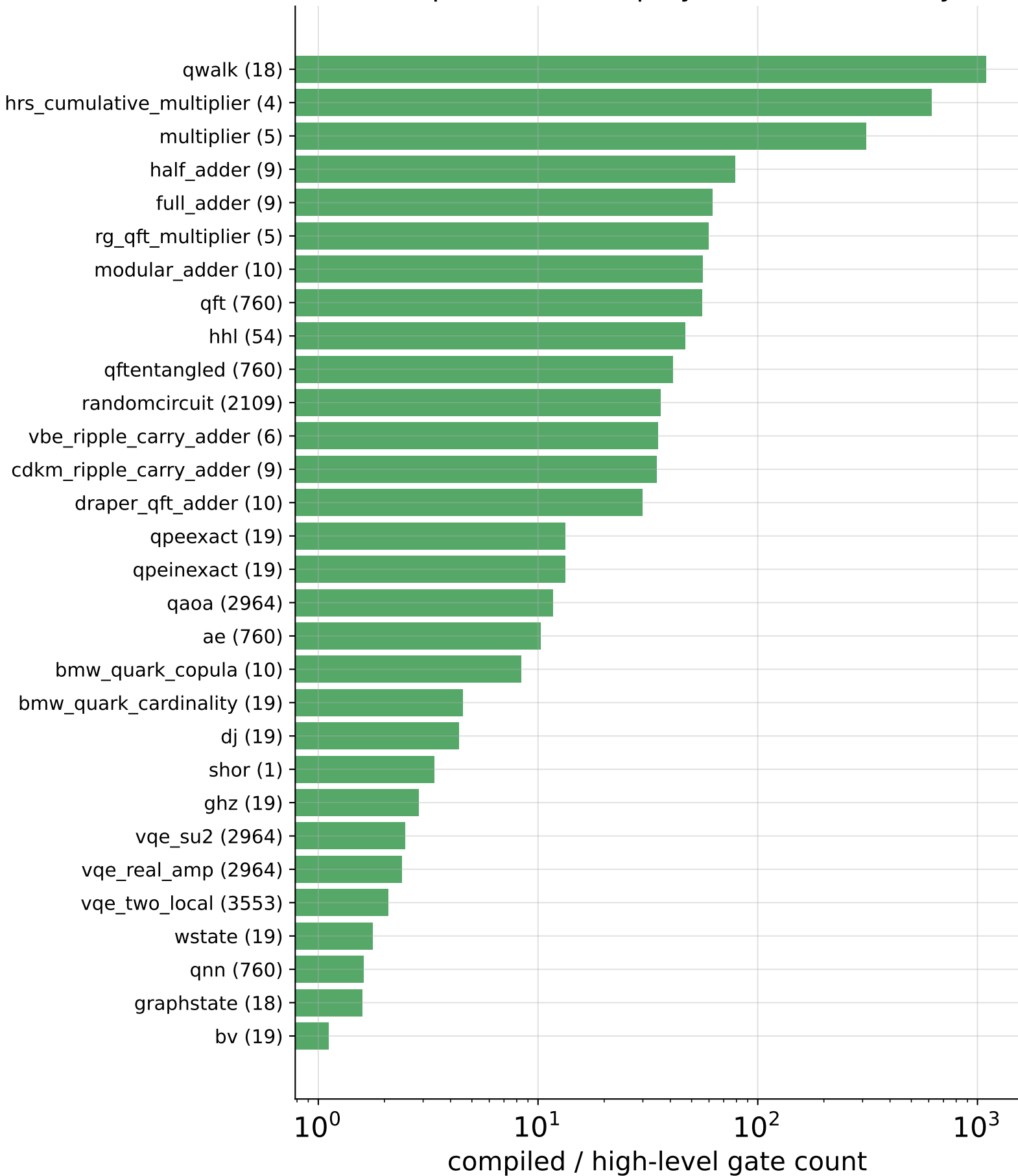
Transpilation blow-up by benchmark family
