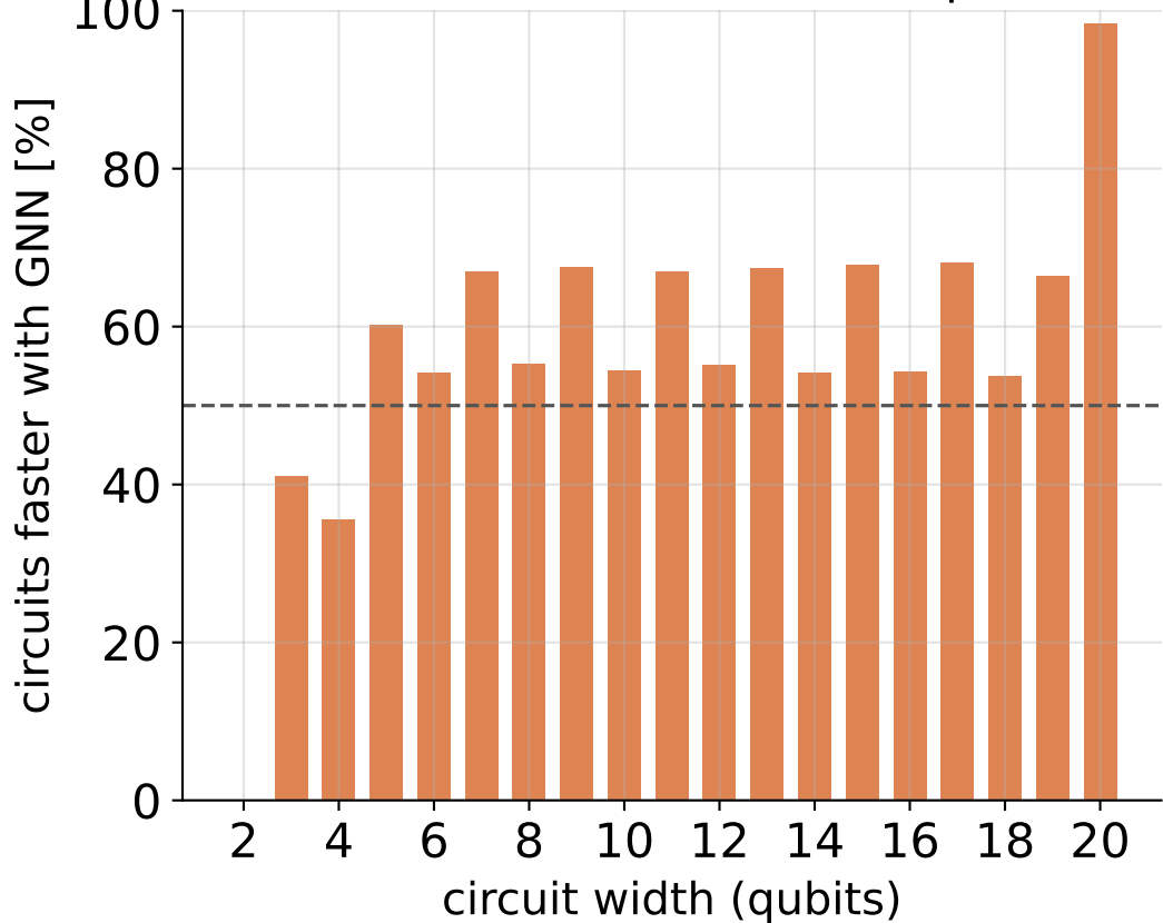
Share of circuits where the GNN path wins
