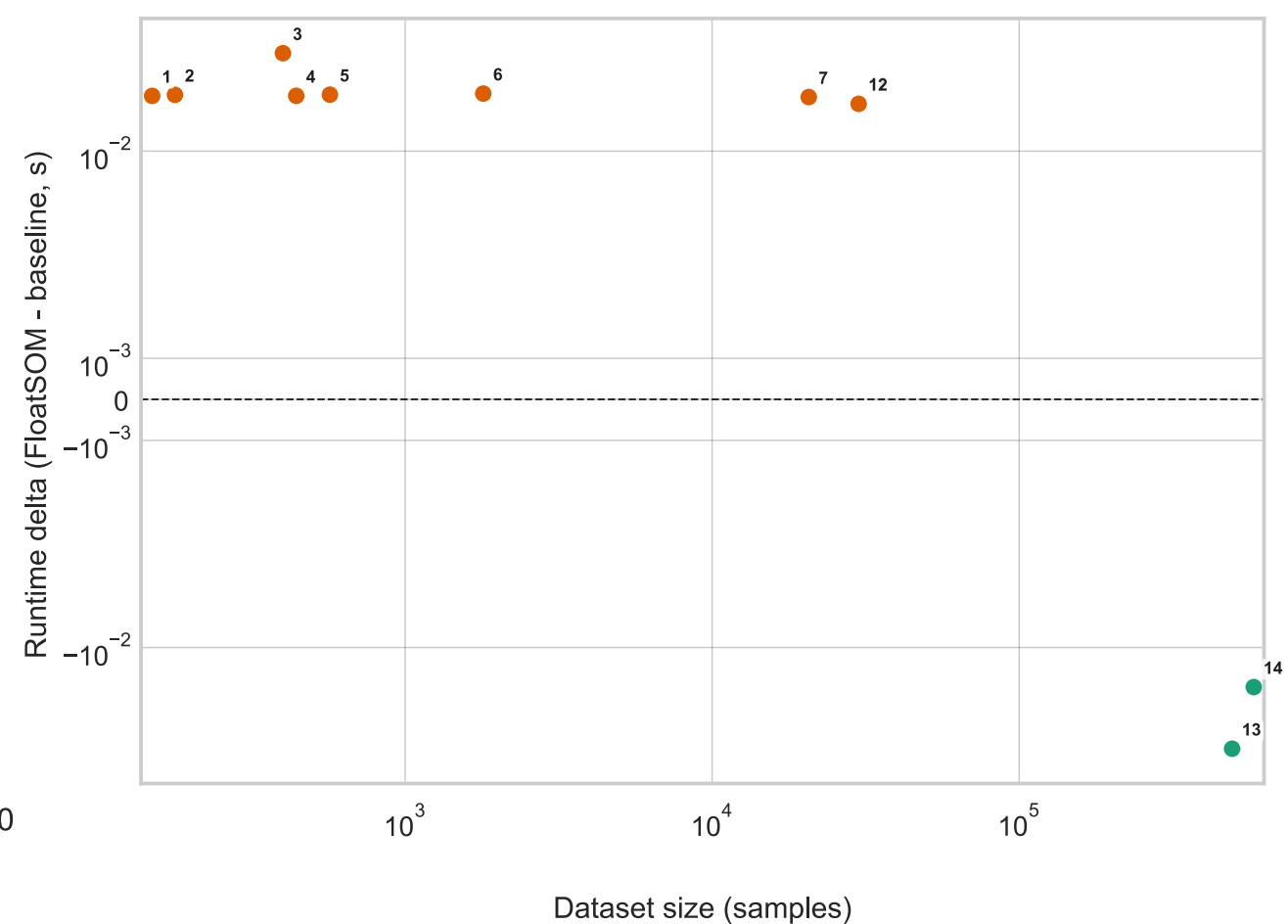
D Runtime Delta vs Dataset Size
