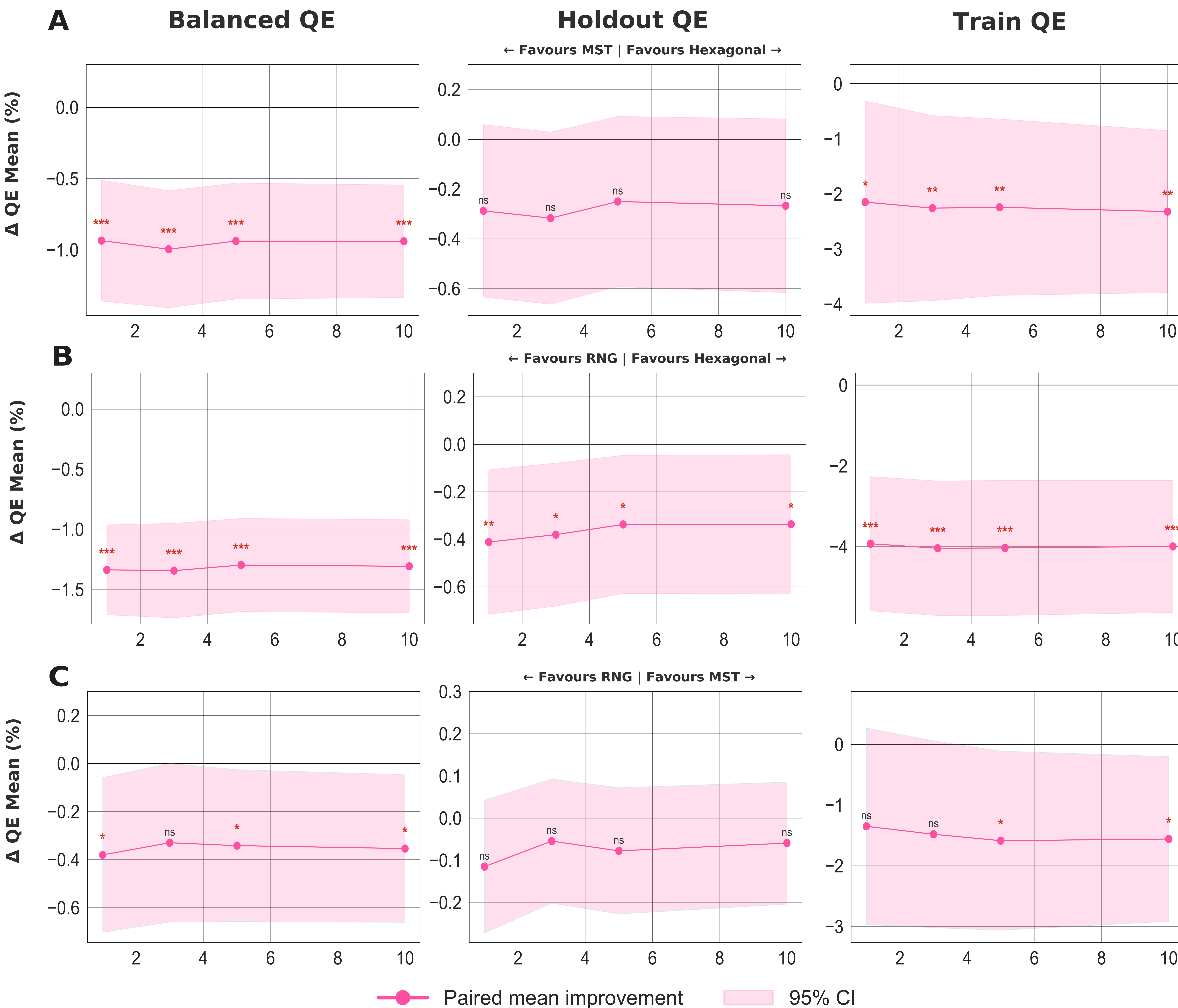
Supplementary Figure S2: Topology Sensitivity by Contrast
