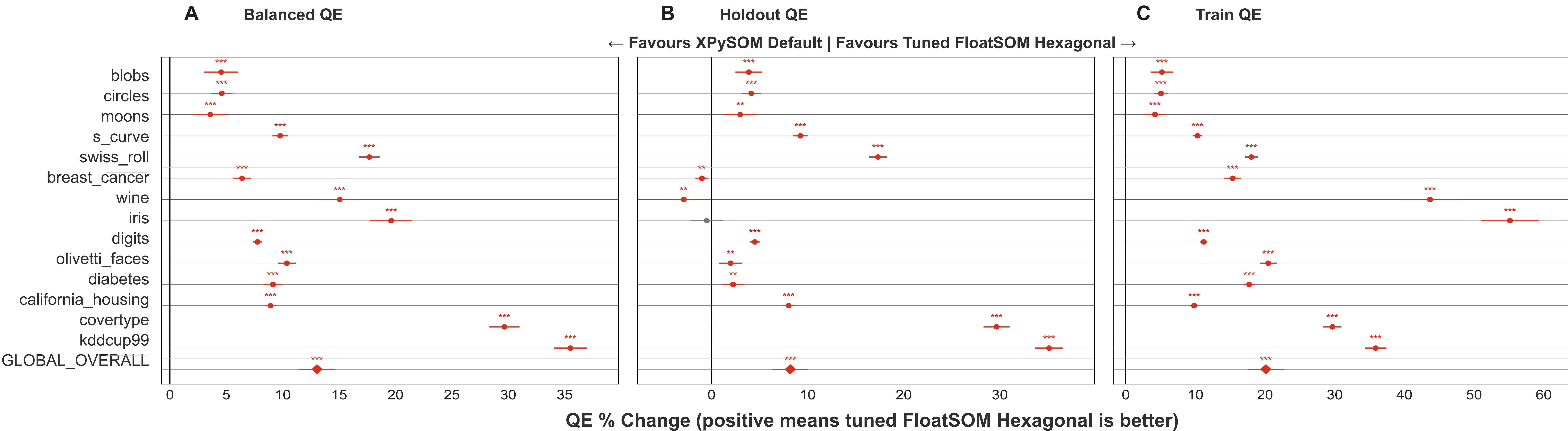
Supplementary Figure S12: XPySOM (Default) v FloatSOM Hexagonal
