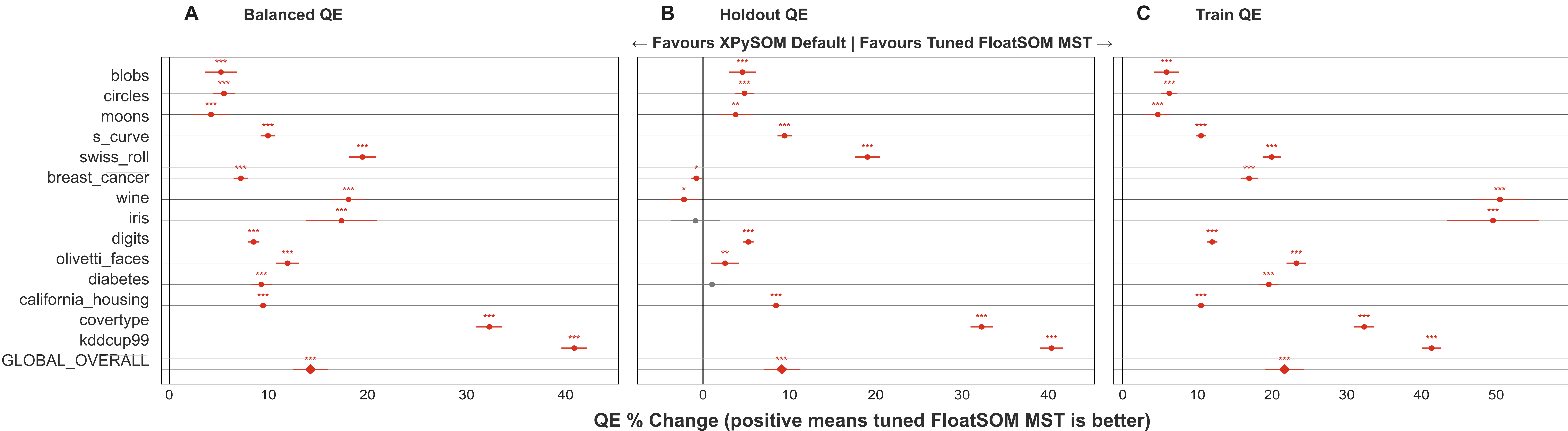
Supplementary Figure S13: XPySOM (Default) v FloatSOM MST
