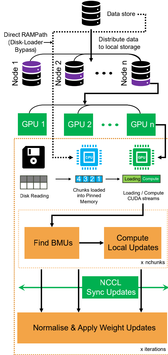
Figure 2: Multi-GPU data loading and NCCL synchronization schematic. In disk-backed mode, data are sharded to worker-local storage, loaded chunk-wise into pinned host memory, transferred to GPU with data transfer overlapping computation, processed locally, and synchronized by NCCL all-reduce before one weight update per iteration. In RAM mode, data are instead pre-sharded into worker-local CPU RAM and follow the same pinned-memory-to-GPU path without disk reads.
