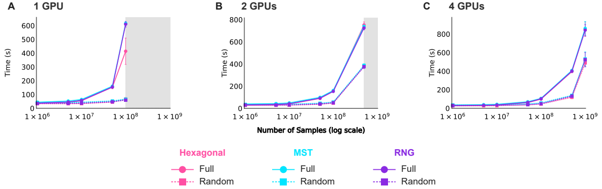
Figure 12: Sampling Runtime
