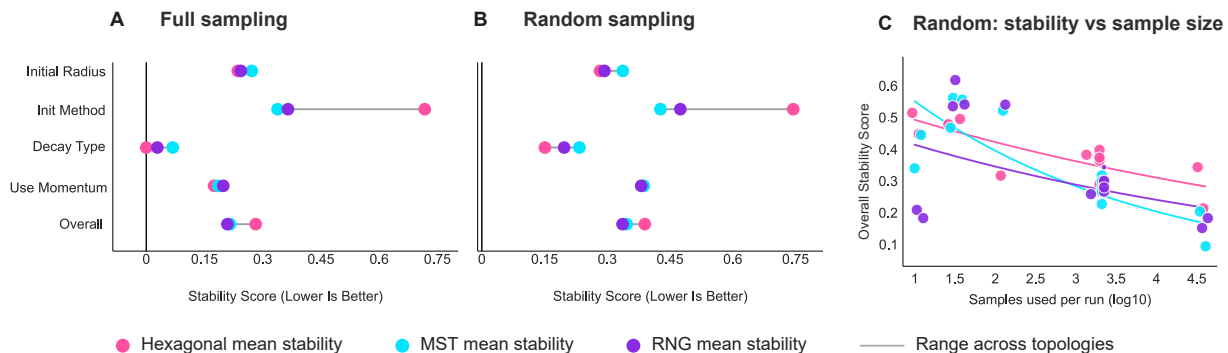
Figure 11: Hyperparameter Stability
