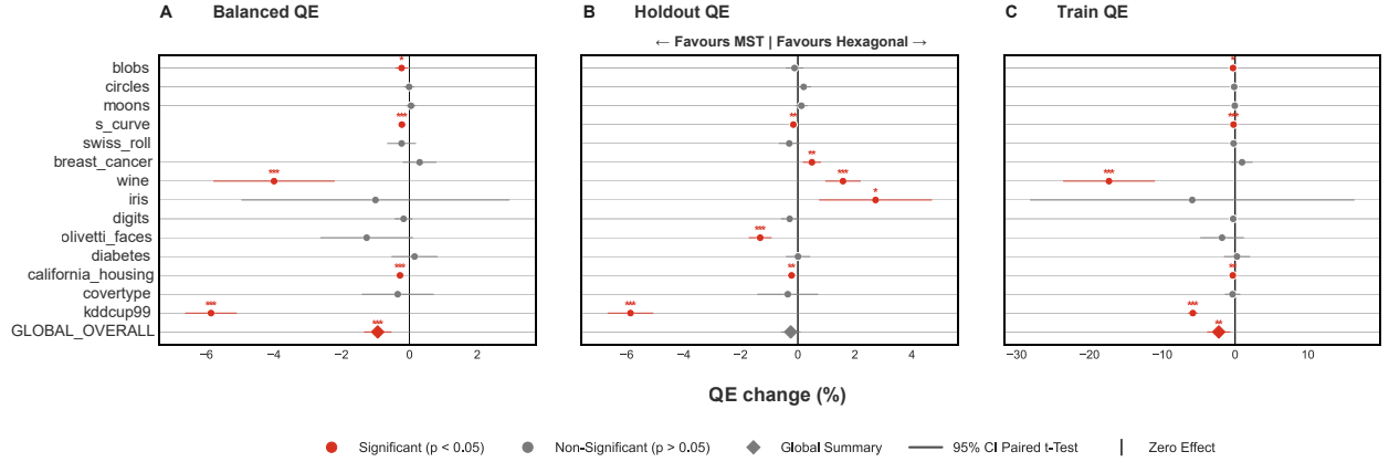
Figure 6: Hexagonal vs MST Across QE Metrics
