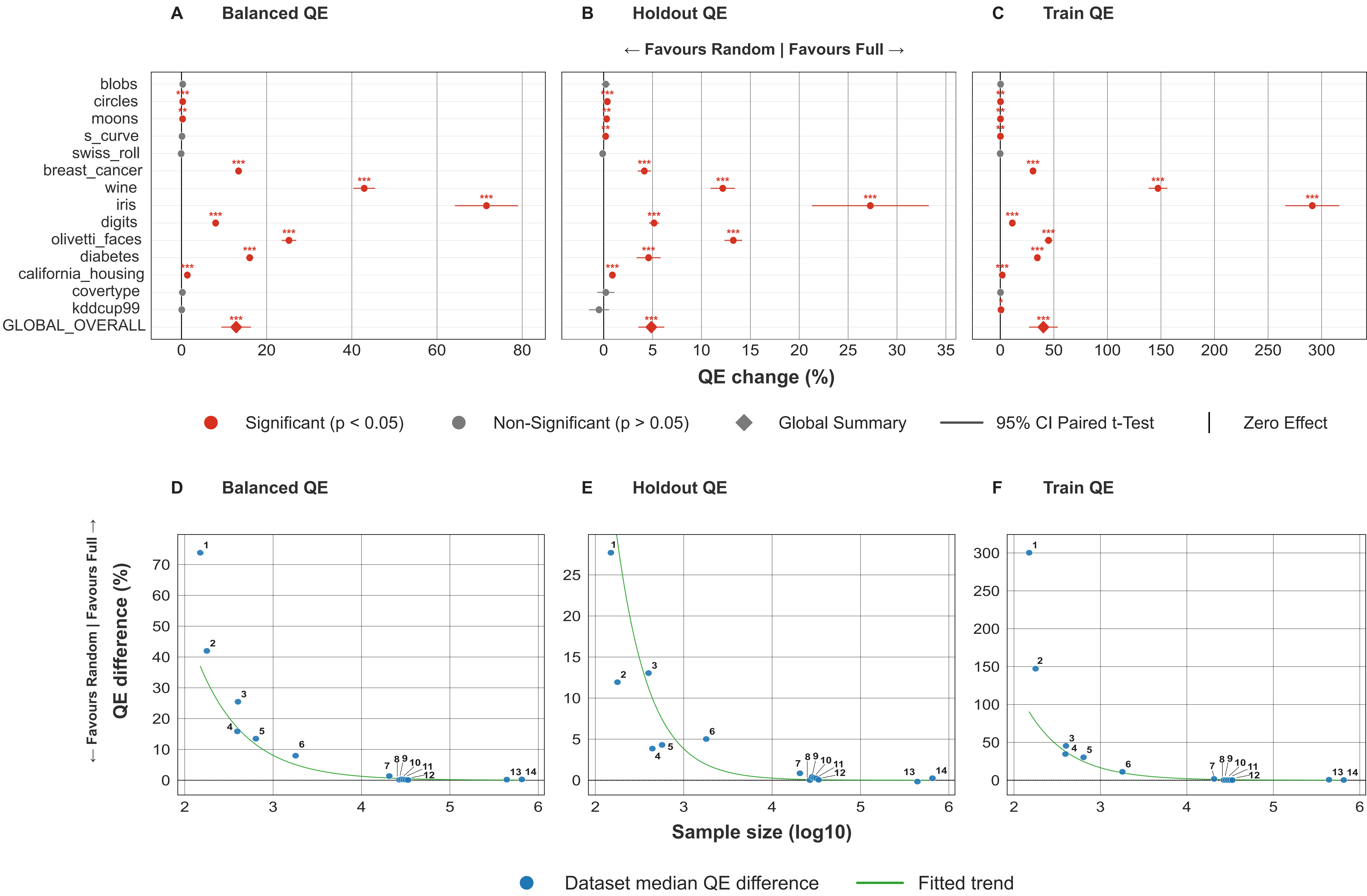
Figure 4: Full vs Random Outcomes and Dataset-Size Regression (Hexagonal / Full Batch)
