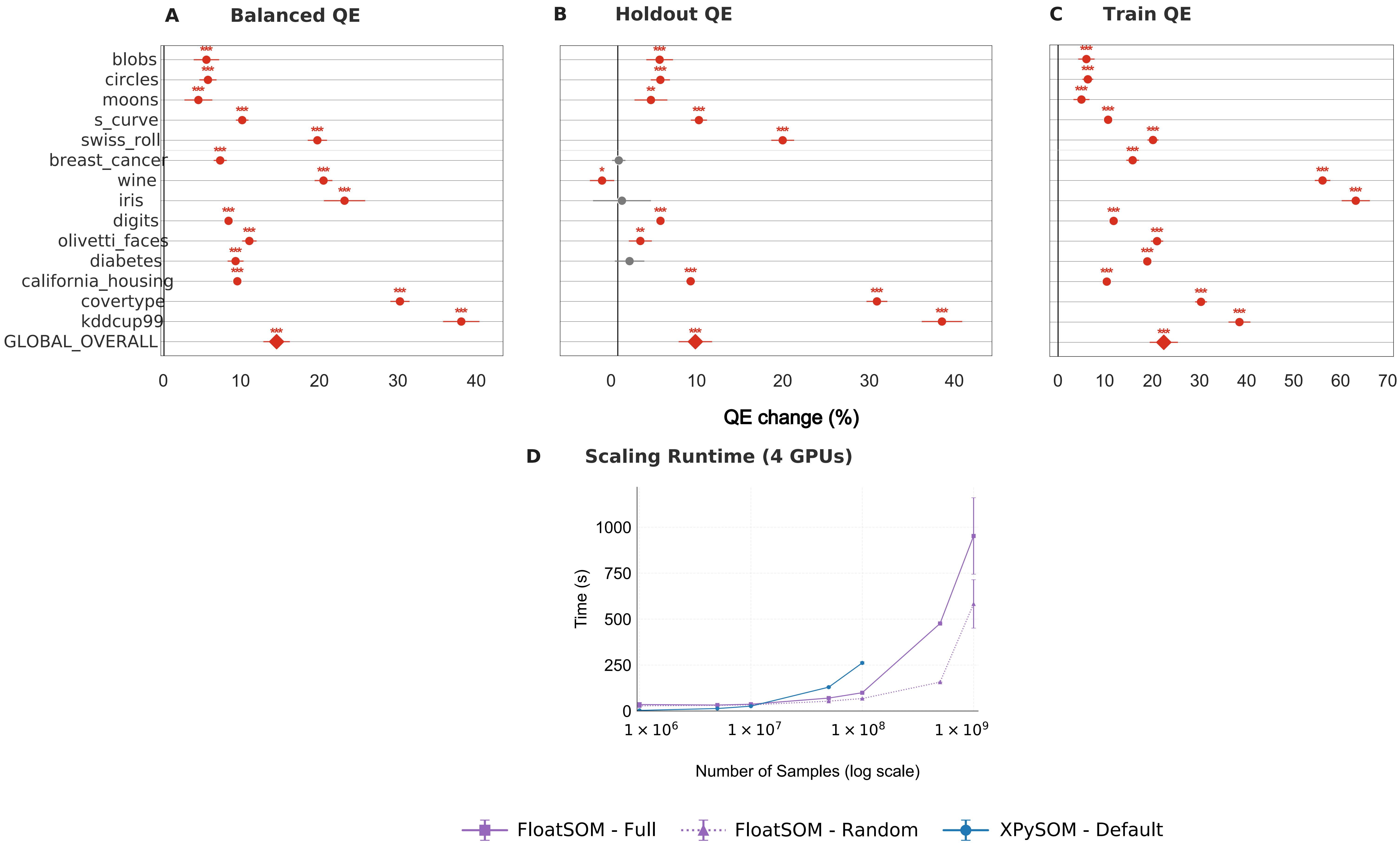
Figure 14: XPySOM (Default) v FloatSOM RNG
