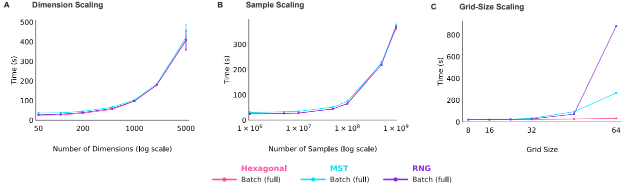
Figure 12: Topology runtime comparison at fixed G = 8 GPUs under full sampling. Panels A-C report mean wall-clock runtime (s) for dimension-, sample-, and grid-size-scaling workloads, respectively, with topology traces for hexagonal, MST, and RNG. Error bars denote \pm 1 standard deviation across n = 3 repeated runs per configuration. The largest-axis 8-GPU topology runtime summaries are listed in Supplementary Table S11.
